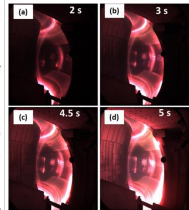
A fast visible wavelength camera's images of plasma inside the EAST Tokamak at various times. DOI:10.1088/1741-4326/ab2c3c
